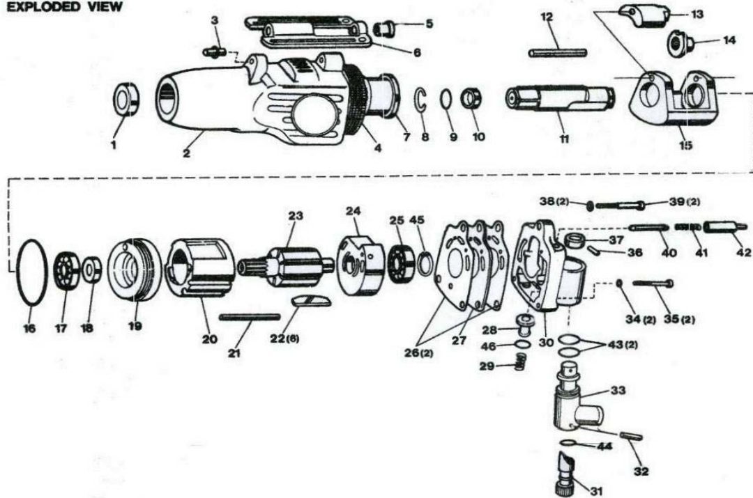
EXPLODED VIEW
